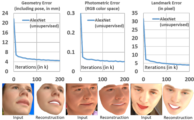
Fig. 14. Quantitative evaluation of MoFA on synthetic ground truth data: Training decreases the geometric, photometric and landmark error.
