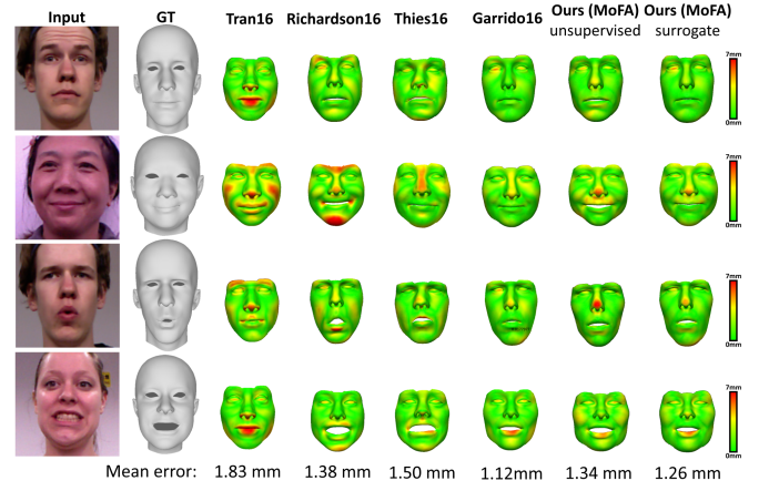
Fig. 15. Quantitative evaluation on Facewarehouse [71]: We obtain a low error that is comparable to optimization-based approaches. For this test, we trained our network using the intrinsics of the Kinect.
