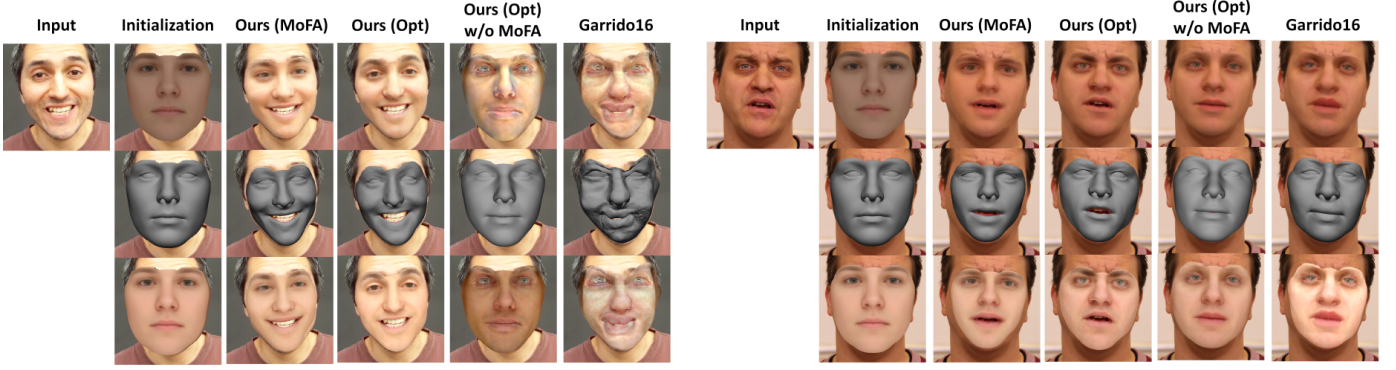
Fig. 18. Qualitative comparison between MoFA and MoFA with analysis-by-synthesis optimization (Opt) without the landmark term. Opt improves the MoFA estimates while Garrido et al. [8], which starts from a neutral initialization (second column), often ends up in local minima in the absence of landmarks. Opt, when starting from a neutral initialization also fails to estimate plausible reconstructions.
