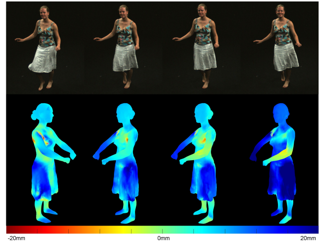
Fig. 16. Improvement of the non-rigid stage ( E_{pose} + E_{non-rigid} ) over pose-only deformation ( E_{pose} ). Top row: Four monocular input images. On the bottom row, for each image, we show the per-vertex error of the pose only results minus the per-vertex error of our method. Consequently, negative means pose only is better and is colored in red. Positive means our method is better and is colored in blue. As expected our method achieves most improvement on the non-rigid skirt part— which is around 20mm for the shown frames.
