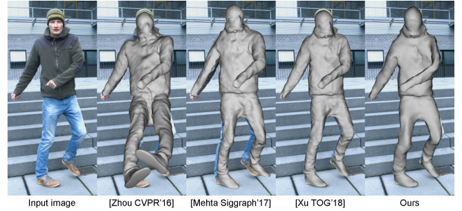
Fig. 7. Qualitative comparison to related monocular methods. The results of our approach overlay much better with the input than the skeleton-only results of Zhou et al. [2016] and Mehta et al. [2017]. Our results come close in quality to the off-line approach of Xu et al. [2018].
