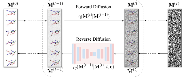
Figure 2: An illustration of our diffusion for 3D human motion synthesis. During forward diffusion, we iteratively add Gaussian noise q(M^{(t)}|M^{(t-1)}) = \mathcal{N}(M^{(t)}|(1 - \beta_t)M^{(t-1)}, \beta_t I) to initial motion at t = 0 . A neural network f_{\theta}(\cdot, \cdot) is trained to denoise the noisy motion M^{(t)} at time t based on the conditioning signal c .
