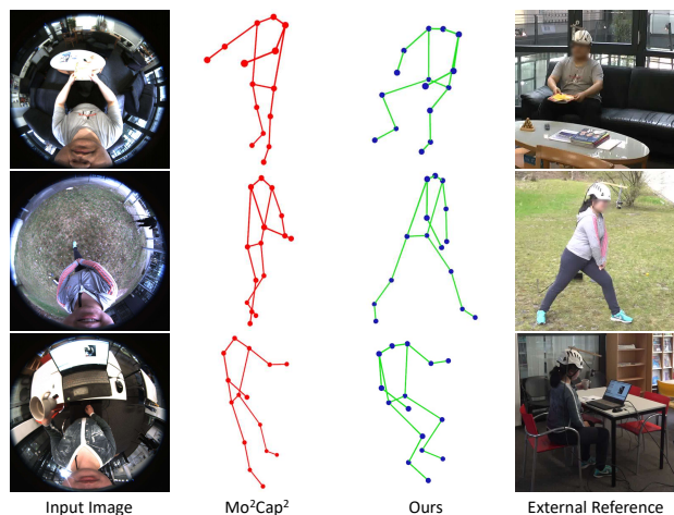
Figure 1. Compared with Mo 2 Cap 2 , our method gets a more accurate egocentric pose from a single in-the-wild image, especially when the body parts are occluded. Note that the external images are only used for visualization, not the inputs to our method.
